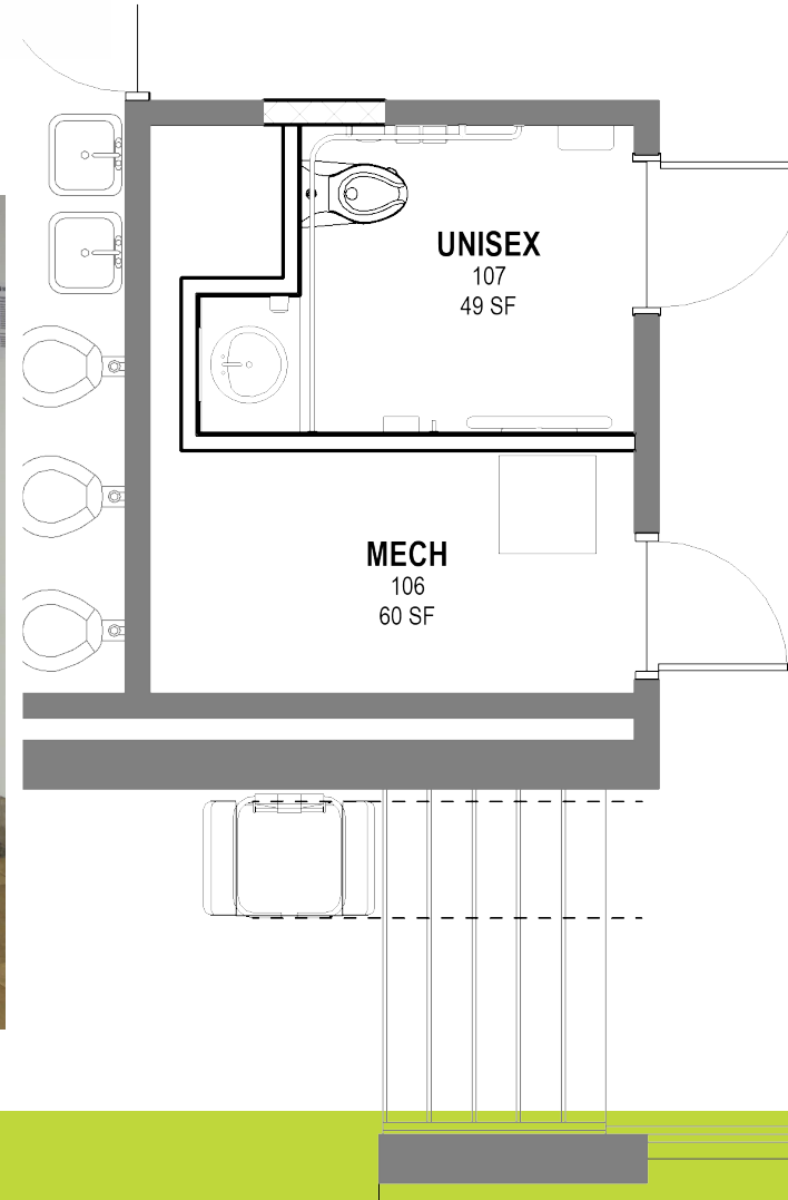
ENLARGED PLAN OF PLATFORM LIFT & RESTROOM
